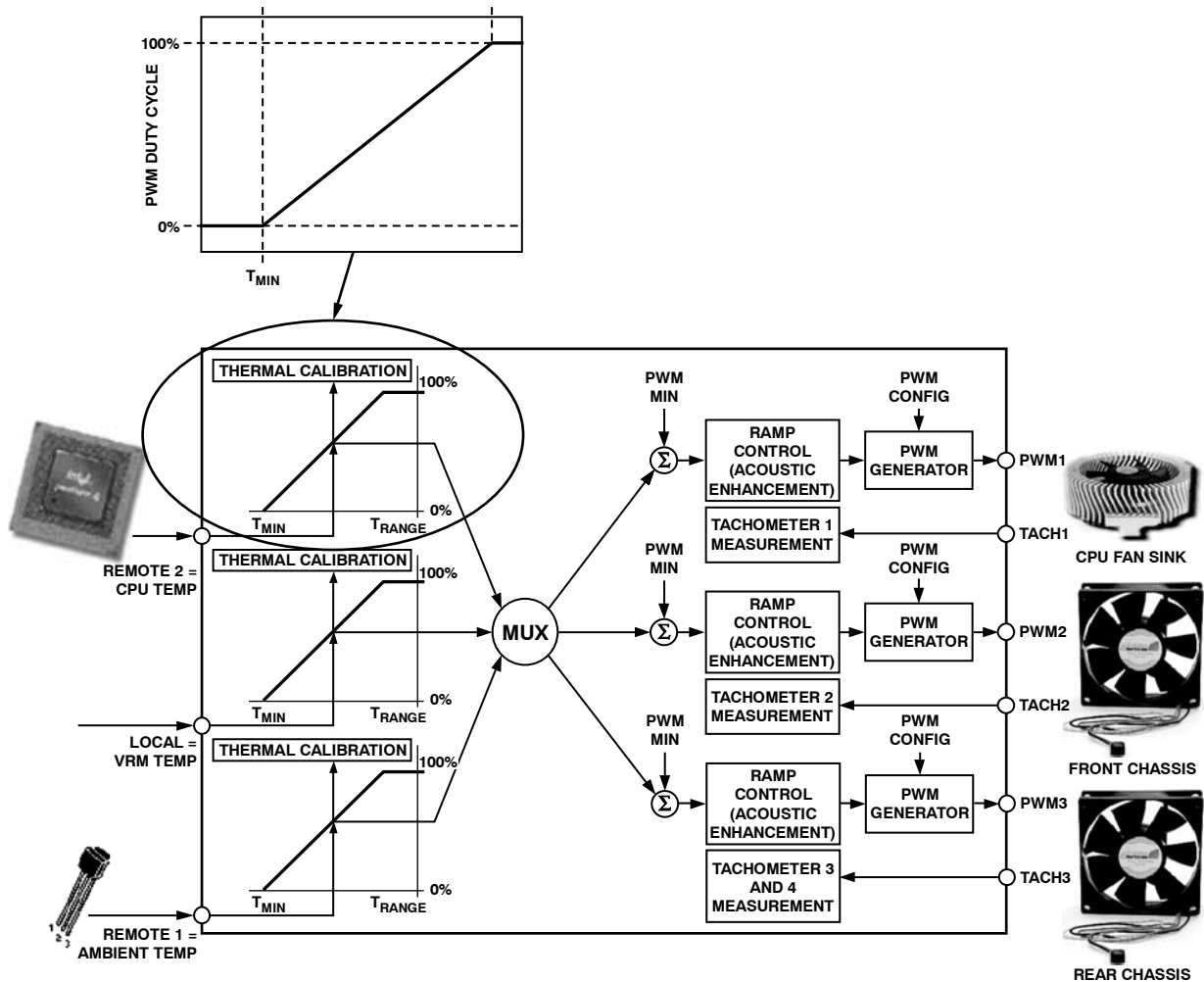
Figure 54. Understanding the T MIN Parameter
