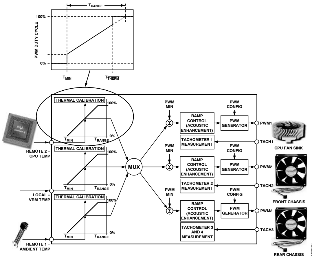
Figure 64. How T_{THERM} Relates to Automatic Fan Control
