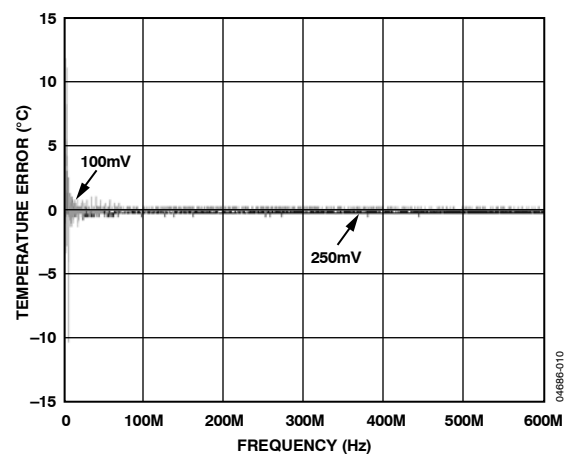
Figure 10. Internal Temperature Error vs. Frequency
