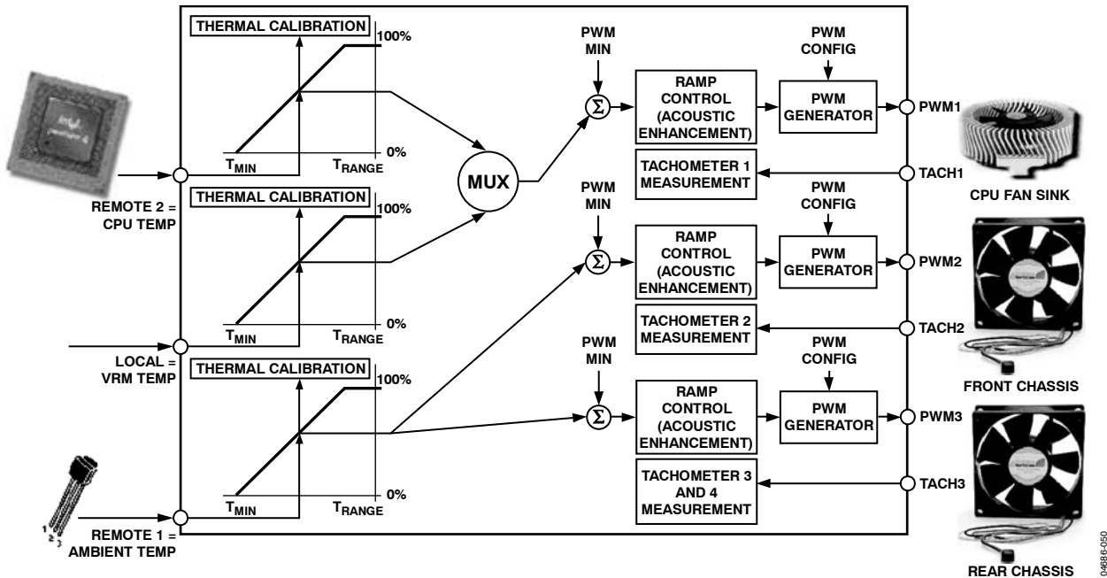
Figure 53. Mux Configuration Example
