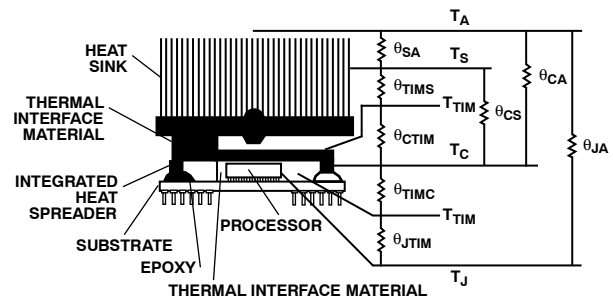
Figure 67. Thermal Model
