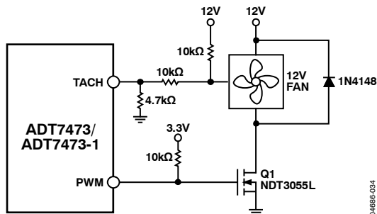
Figure 37. Driving a 3-Wire Fan Using an N-Channel MOSFET
