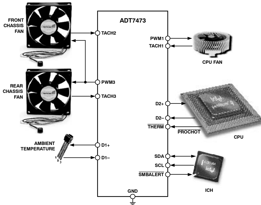
Figure 51. Recommended Implementation 1
