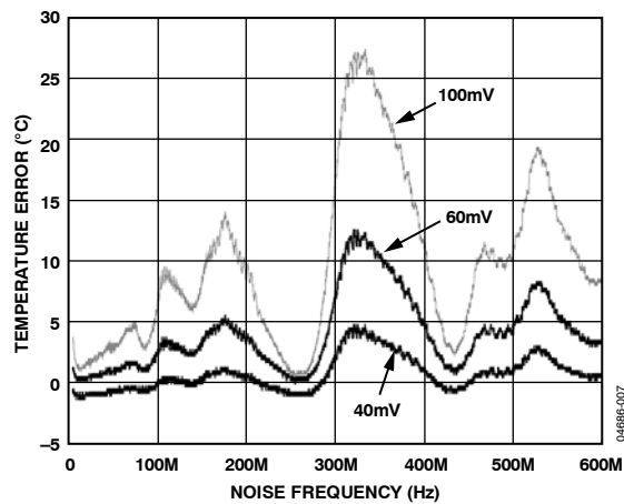
Figure 7. Remote Temperature Error vs. Common-Mode Noise Frequency
