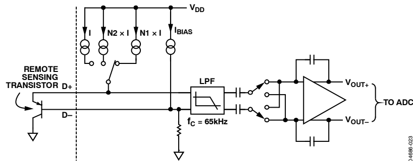
Figure 26. Signal Conditioning for Remote Diode Temperature Sensors
