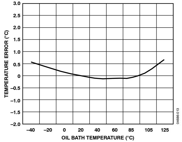
Figure 13. Remote Temperature Error vs. Temperature
