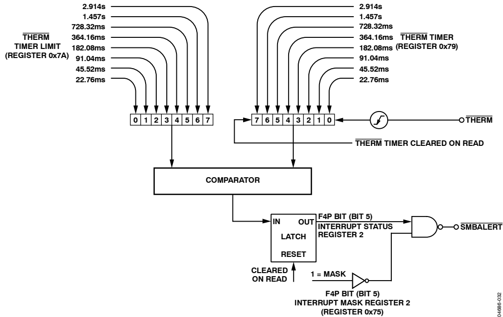
Figure 35. Functional Block Diagram of the ADT7473 THERM Monitoring Circuitry
