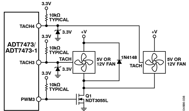
Figure 42. Fan with TACH Pull-Up to V_{CC}
