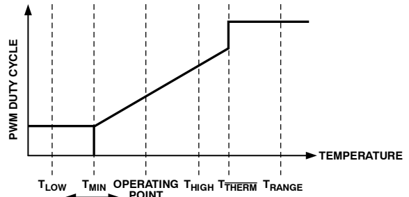
Figure 68. Dynamic T_{MIN} Control Loop
