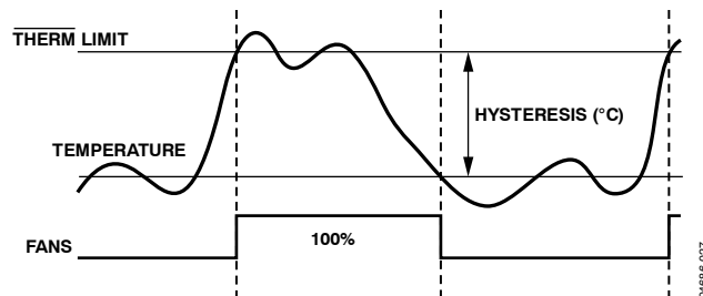
Figure 30. THERM Limit Operation
