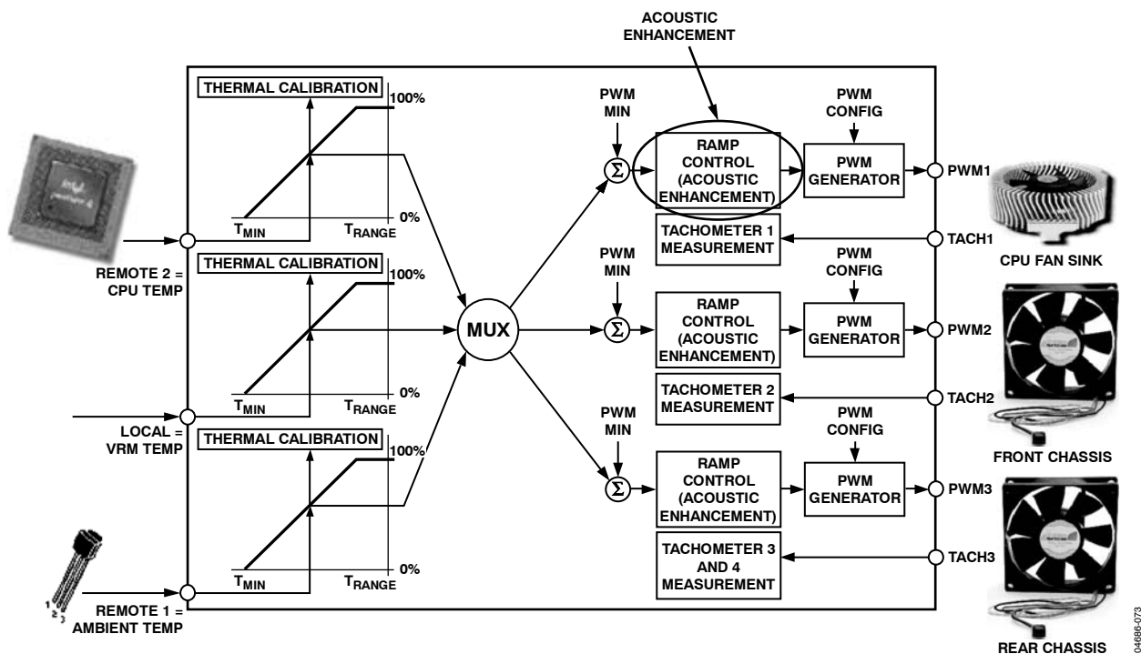
Figure 76. Acoustic Enhancement Smooths Fan Speed Variations Under Automatic Fan Speed Control
