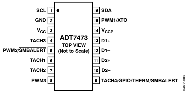
Figure 3. ADT7473 Pin Configuration
