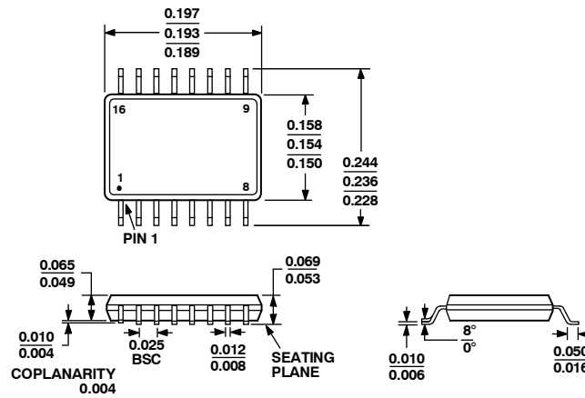
Figure 84. 16-Lead Shrink Small Outline Package [QSOP] (RQ-16)
