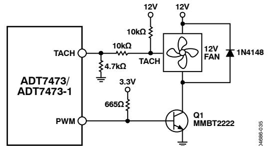
Figure 38. Driving a 3-Wire Fan Using an NPN Transistor
