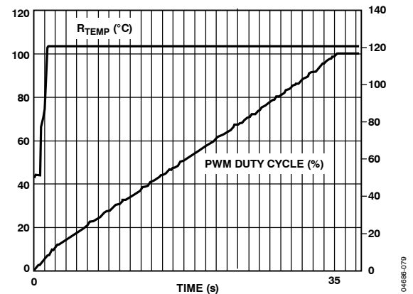
Figure 82. Enhanced Acoustics Mode with Ramp Rate = 1
