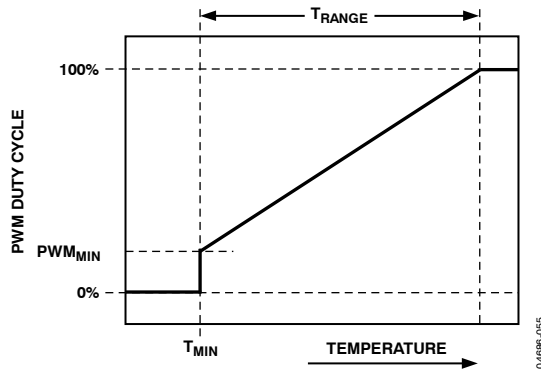
Figure 58. T RANGE Parameter Affects Cooling Slope
