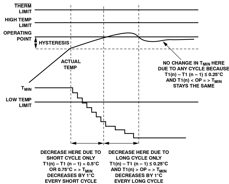
Figure 73. Effect of Exceeding Operating Point Minus Hysteresis Temperature
