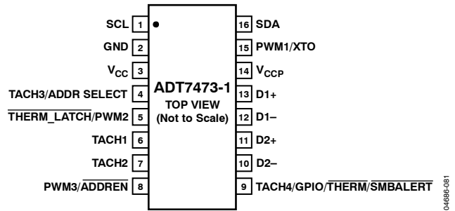
Figure 4. ADT7473-1 Pin Configuration
