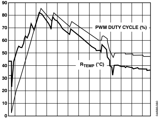
Figure 83. How Fan Reacts to Temperature Variation in Enhanced Acoustics Mode
