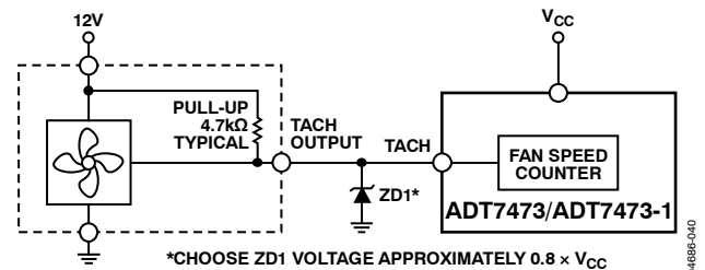
Figure 43. Fan with TACH Pull-Up to Voltage > 3.6 V Clamped with Zener Diode
