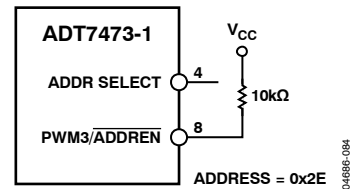
Figure 15. Default SMBus Address = 0x2E
