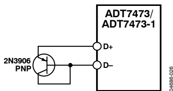
Figure 28. Measuring Temperature Using a PNP Transistor
