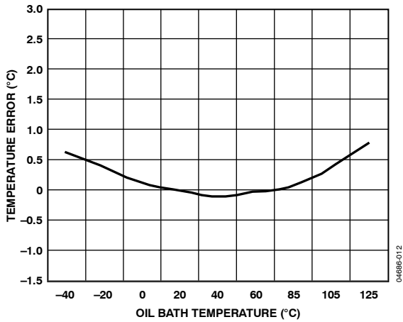
Figure 12. Internal Temperature Error vs. Temperature
