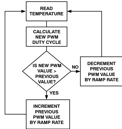
Figure 78. Enhanced Acoustics Algorithm
