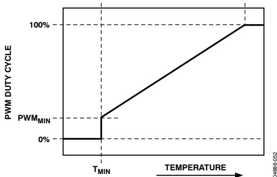
Figure 55. PWM MIN Determines Minimum PWM Duty Cycle
