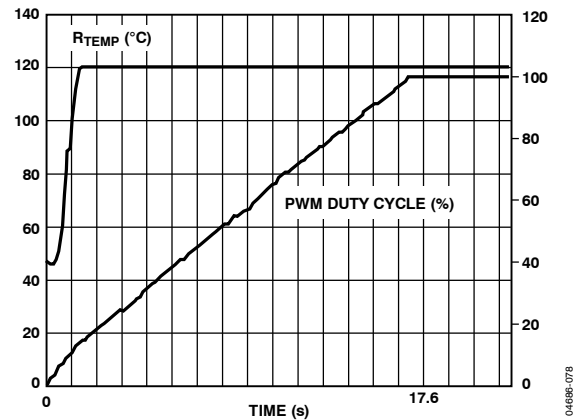
Figure 81. Enhanced Acoustics Mode with Ramp Rate = 2
