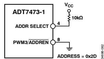
Figure 17. SMBus Address = 0x2D (Pin 4 = 1)
