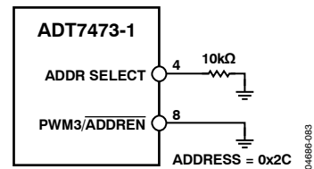
Figure 16. SMBus Address = 0x2C (Pin 4 = 0)
