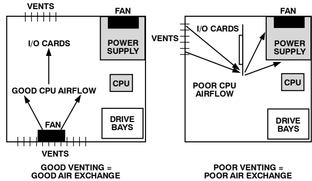
Figure 66. Chassis Airflow Issues
