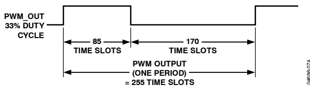
Figure 77. 33% PWM Duty Cycle Represented in Time Slots
