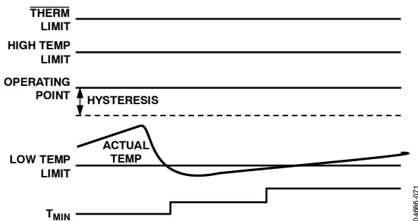
Figure 74. Increasing T_{MIN} for Quieter Operation
