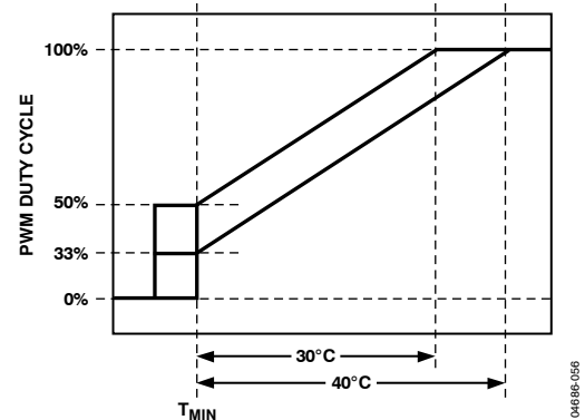
Figure 59. Adjusting PWM MIN Affects T RANGE
