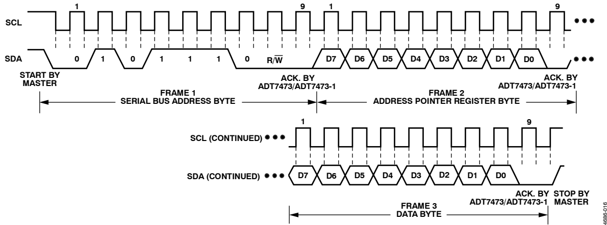
Figure 19. Writing a Register Address to the Address Pointer Register, then Writing Data to the Selected Register
