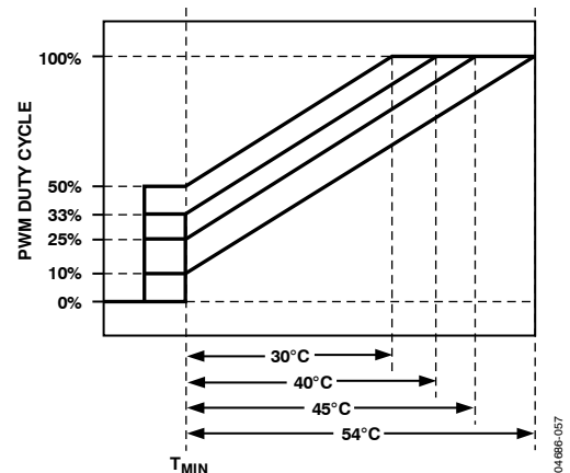
Figure 60. Increasing PWM MIN Changes Effective T RANGE
