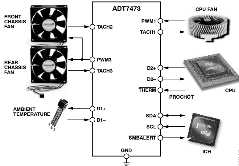
Figure 14. ADT7473 Configuration
