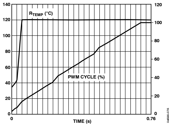
Figure 79. Enhanced Acoustics Mode with Ramp Rate = 48
