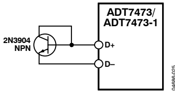
Figure 27. Measuring Temperature Using an NPN Transistor
