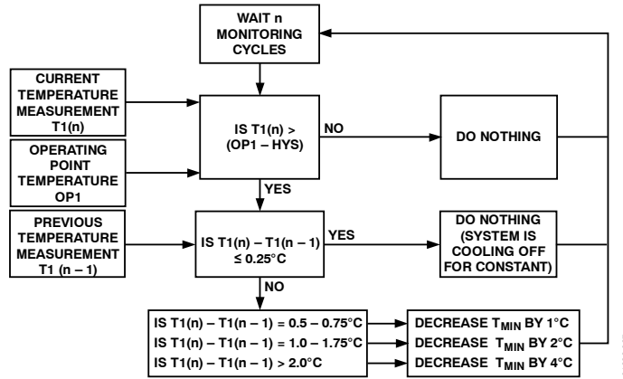
Figure 70. Short Cycle Steps
