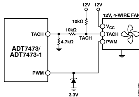
Figure 39. Driving a 4-Wire Fan
