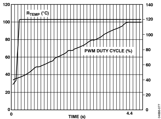
Figure 80. Enhanced Acoustics Mode with Ramp Rate = 8
